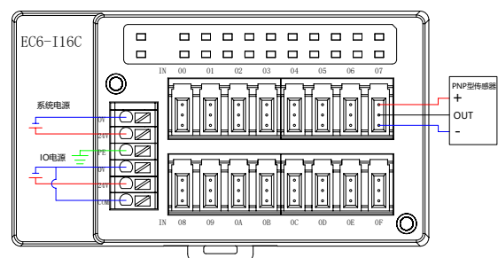
EC6-I16C (PNP输入)
