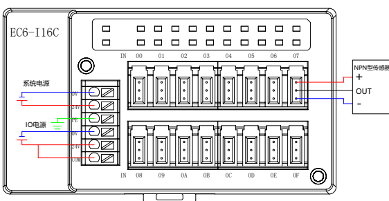
EC6-I16C (NPN输入)
