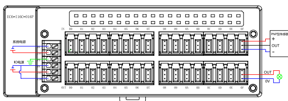
EC6-I16C-O16P (PNP输入, PNP输出)
